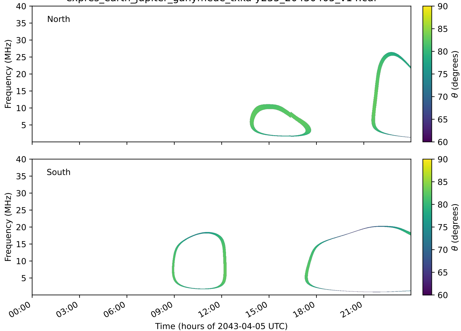
expres_earth_jupiter_ganymede_txka-y235_20430405_v14.cdf
