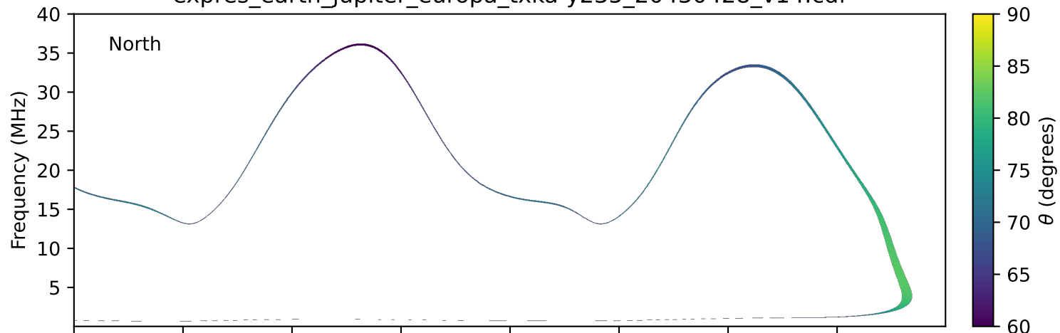
expres_earth_jupiter_europa_txka-y235_20430428_v14.cdf
