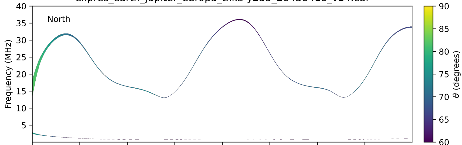
expres_earth_jupiter_europa_txka-y235_20430410_v14.cdf
