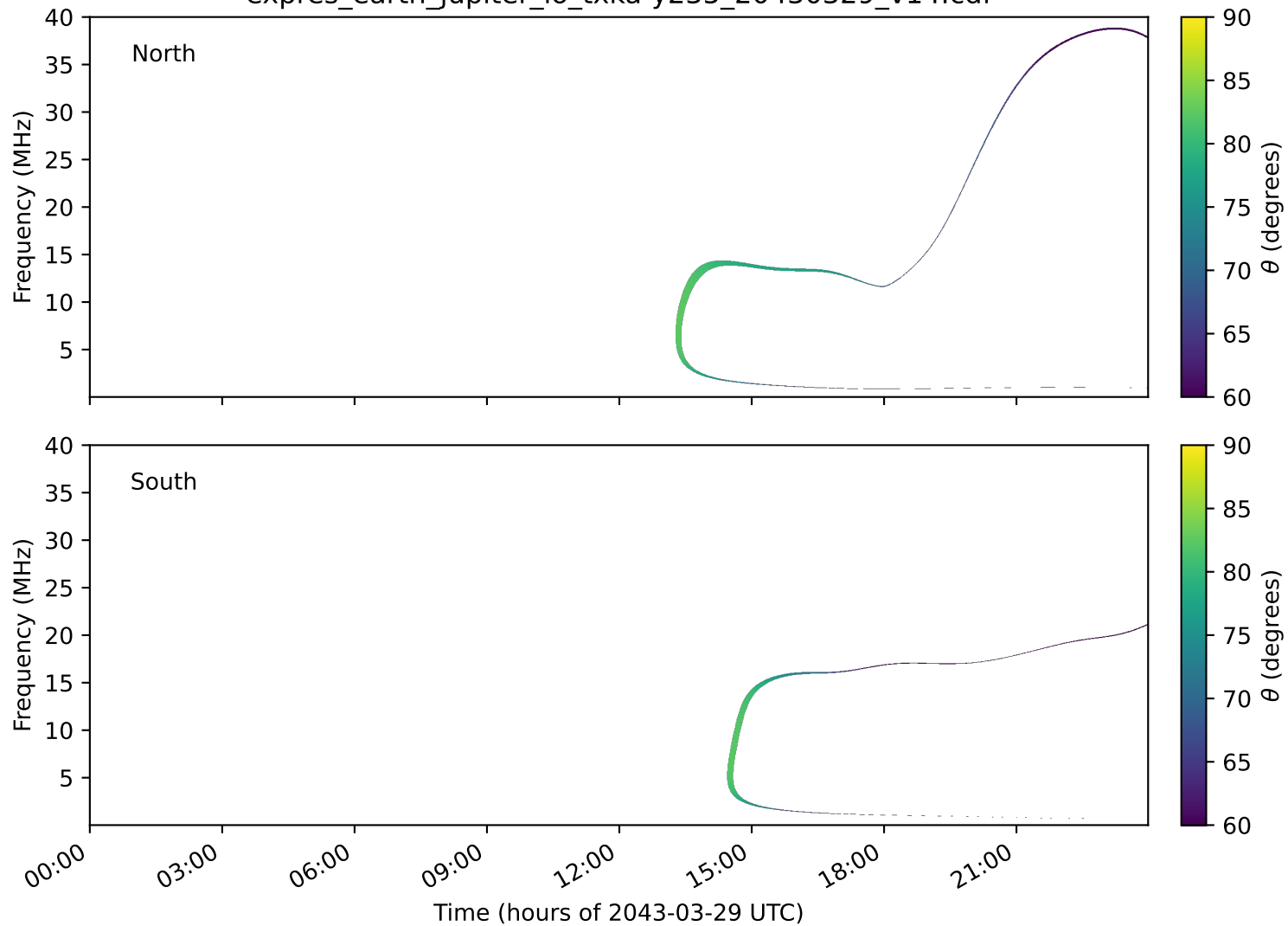
expres_earth_jupiter_io_txka-y235_20430329_v14.cdf
