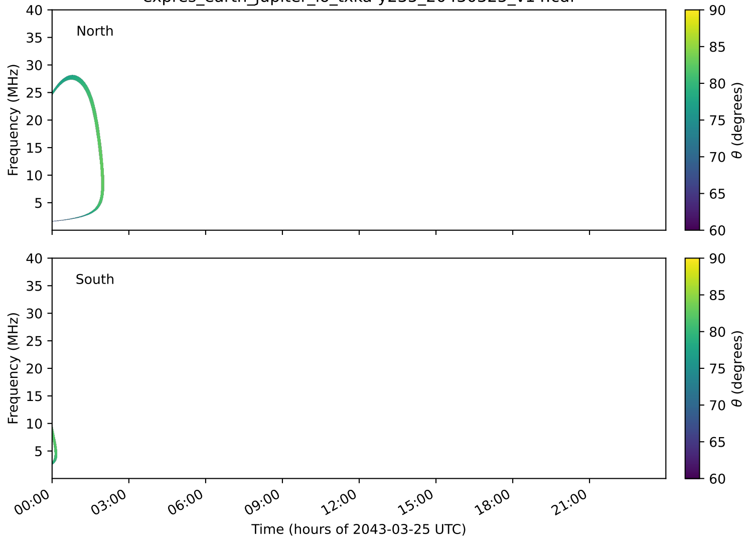
expres_earth_jupiter_io_txka-y235_20430325_v14.cdf
