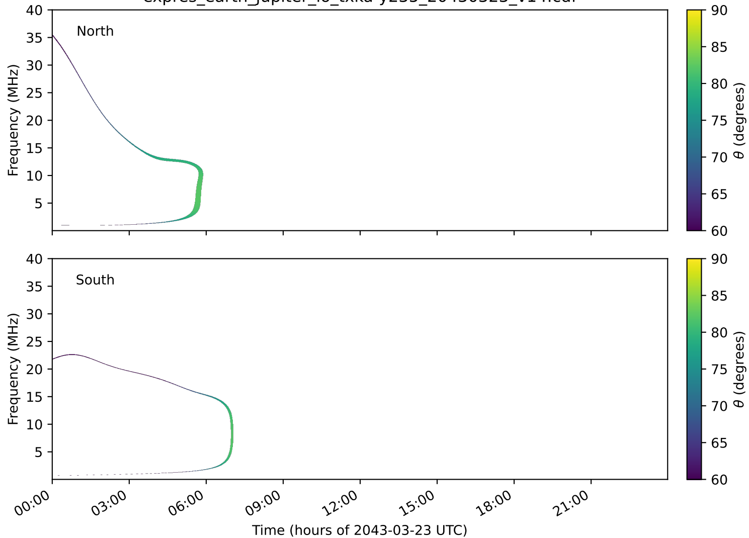
expres_earth_jupiter_io_txka-y235_20430323_v14.cdf
