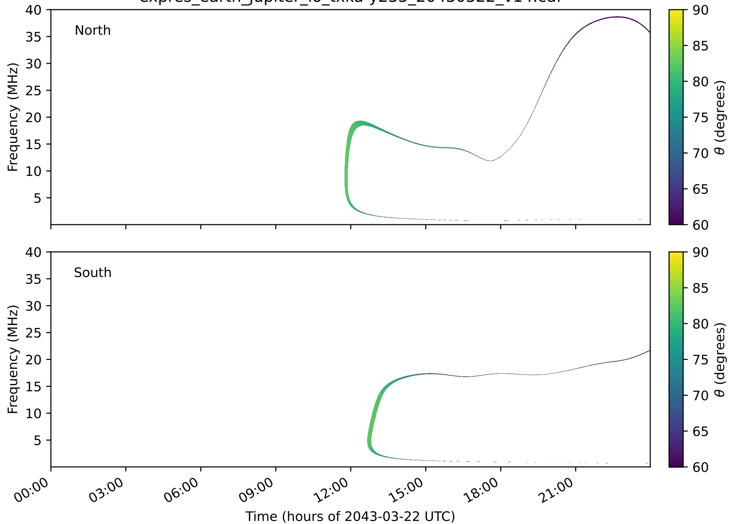
expres_earth_jupiter_io_txka-y235_20430322_v14.cdf
