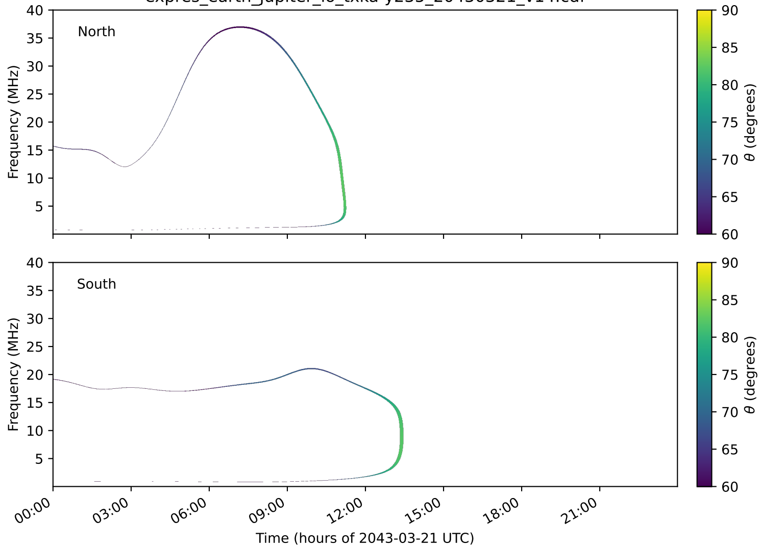
expres_earth_jupiter_io_txka-y235_20430321_v14.cdf
