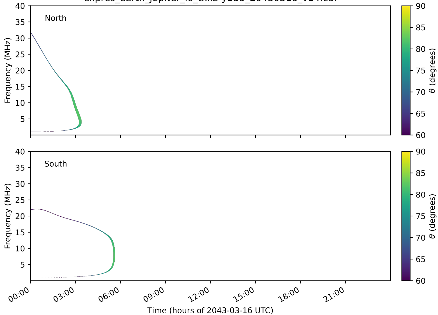
expres_earth_jupiter_io_txka-y235_20430316_v14.cdf
