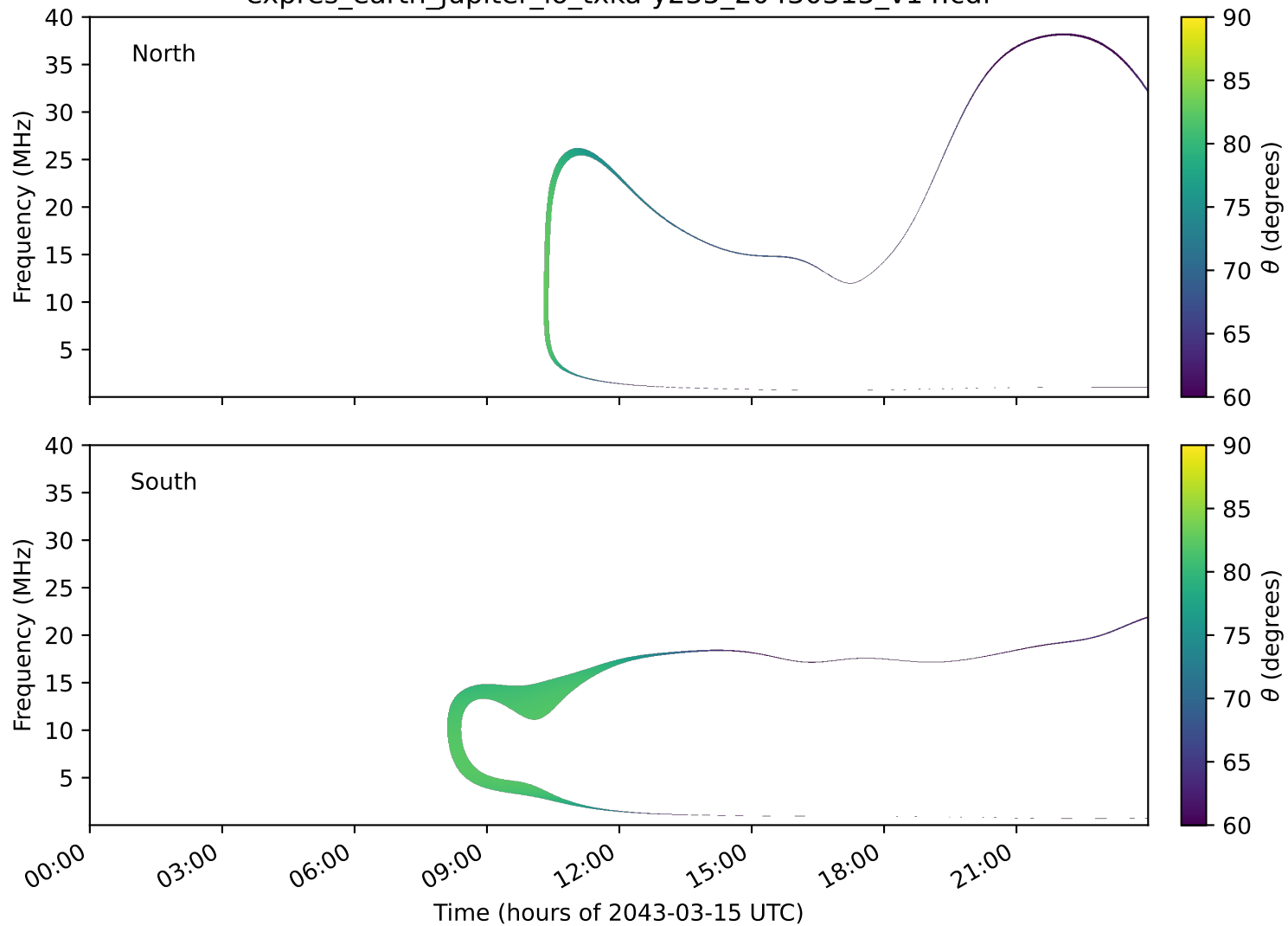
expres_earth_jupiter_io_txka-y235_20430315_v14.cdf
