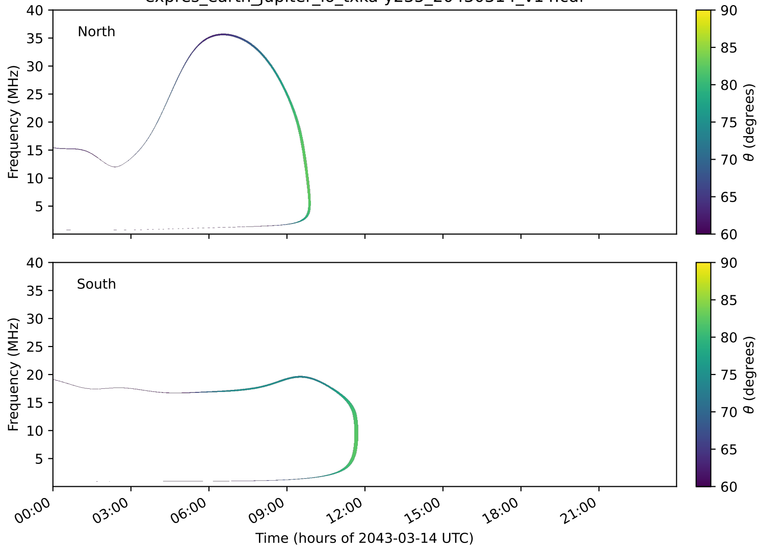
expres_earth_jupiter_io_txka-y235_20430314_v14.cdf
