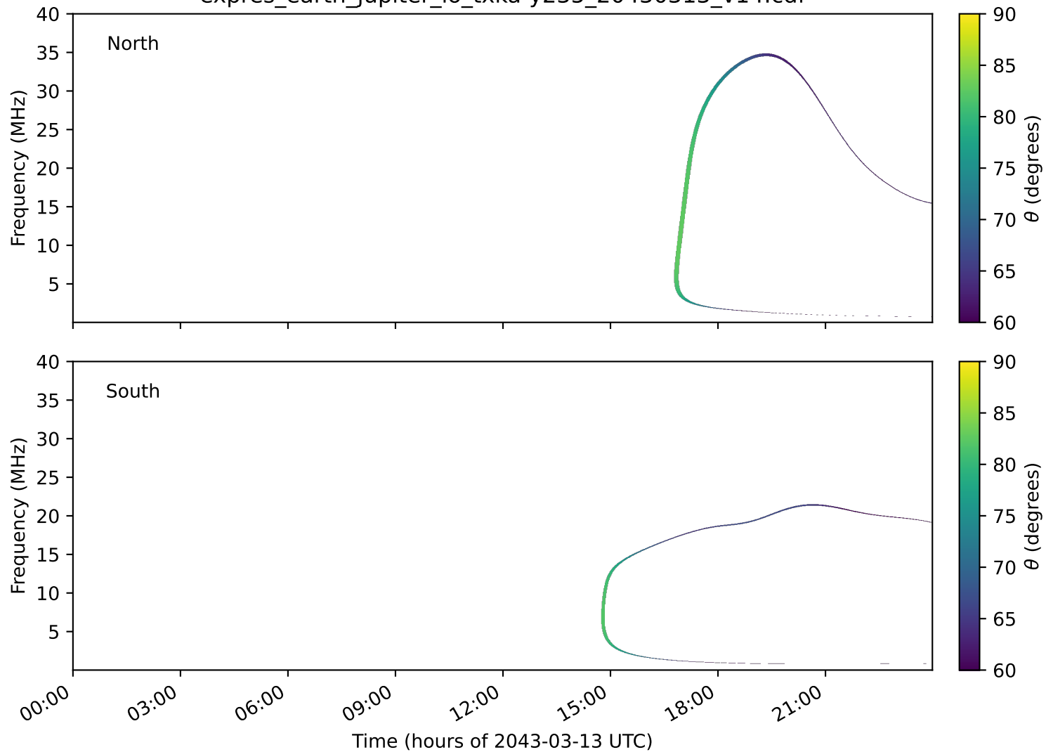
expres_earth_jupiter_io_txka-y235_20430313_v14.cdf
