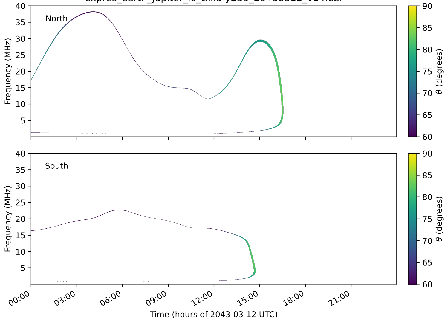
expres_earth_jupiter_io_txka-y235_20430312_v14.cdf
