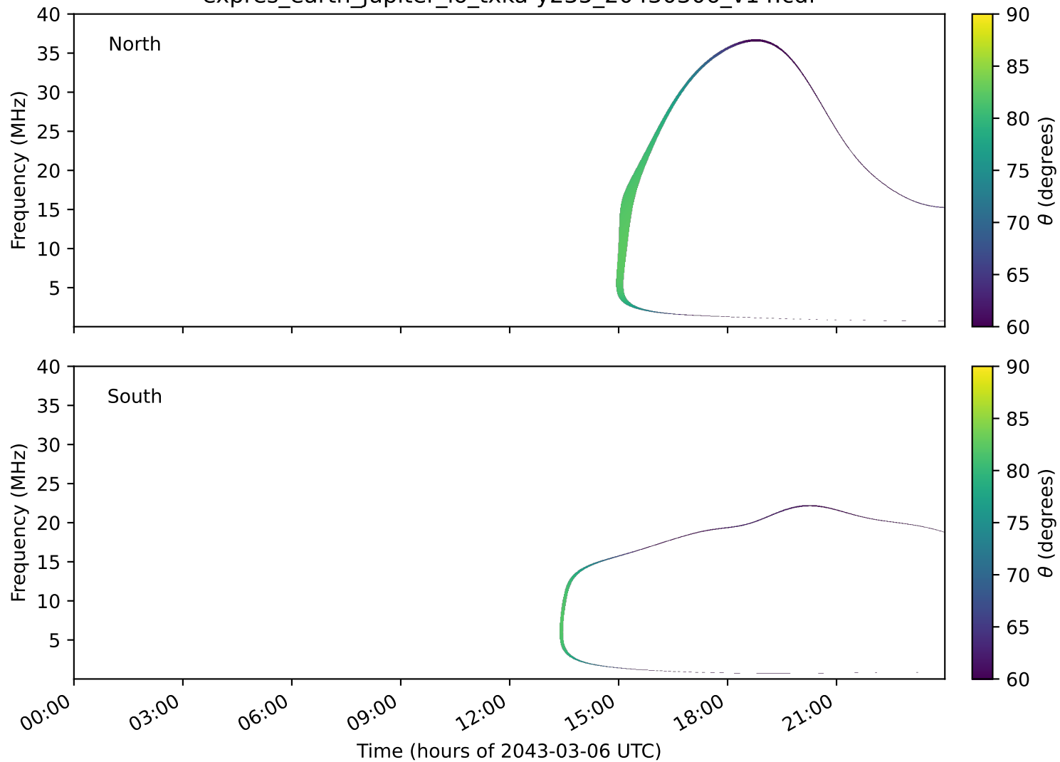
expres_earth_jupiter_io_txka-y235_20430306_v14.cdf
