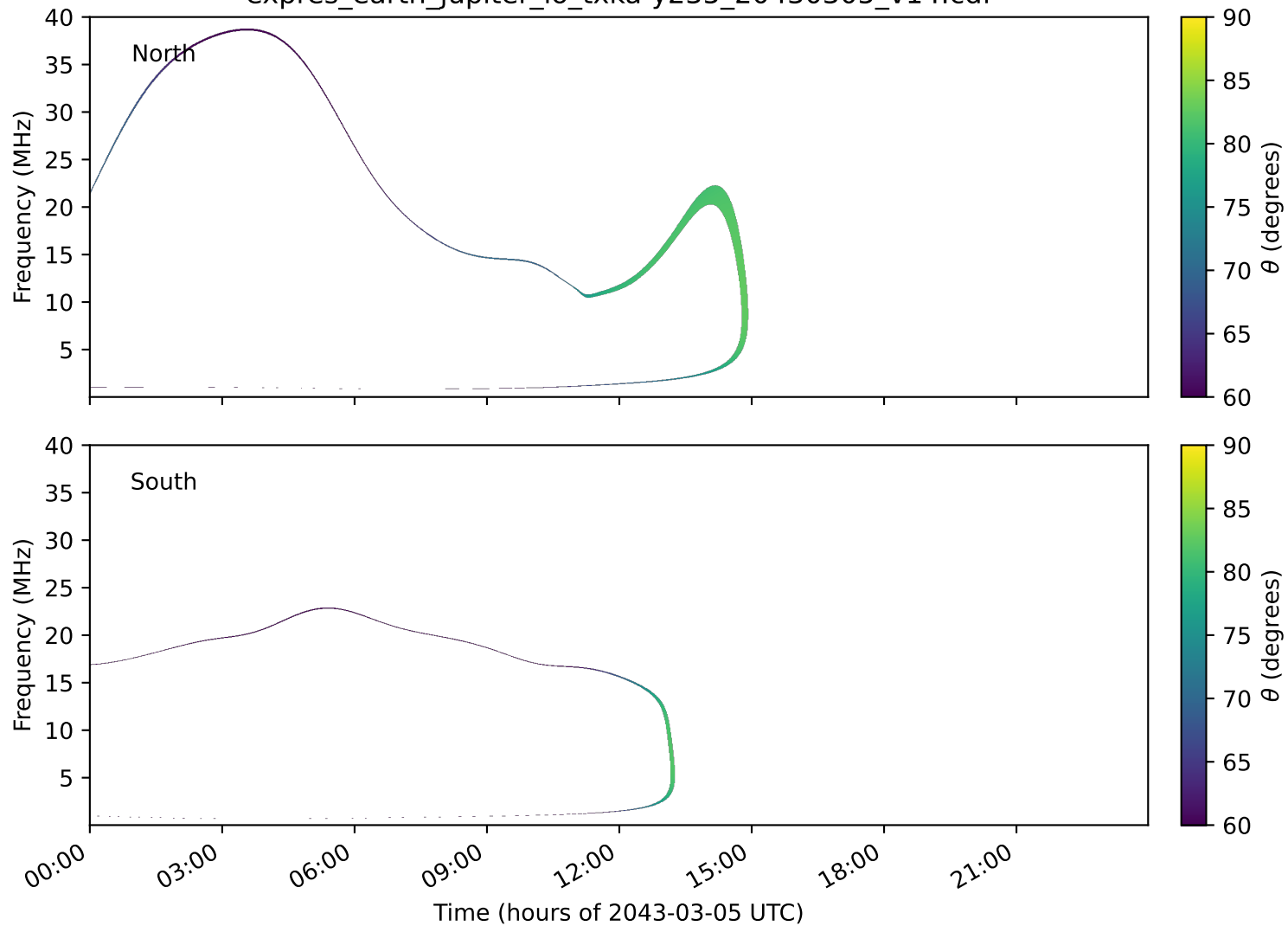
expres_earth_jupiter_io_txka-y235_20430305_v14.cdf
