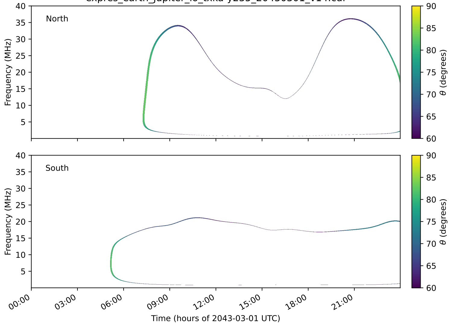
expres_earth_jupiter_io_txka-y235_20430301_v14.cdf
