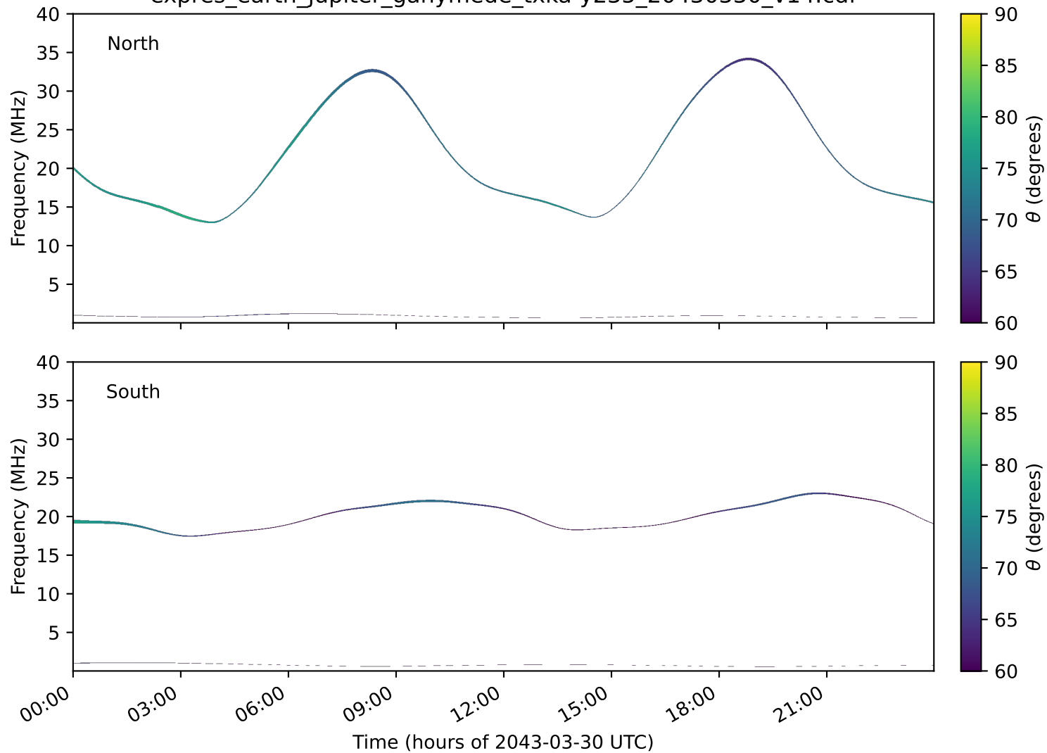
expres_earth_jupiter_ganymede_txka-y235_20430330_v14.cdf
