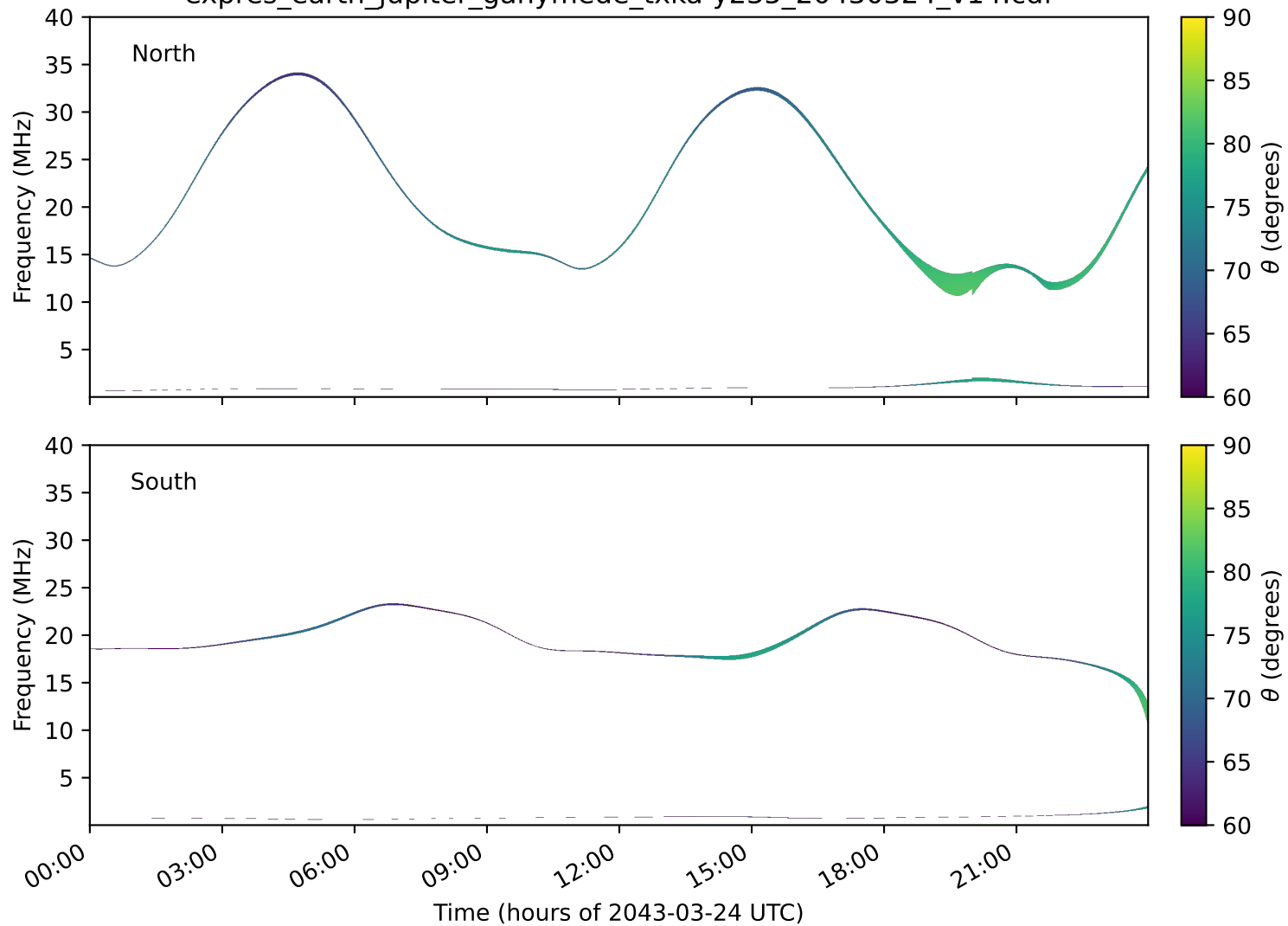
expres_earth_jupiter_ganymede_txka-y235_20430324_v14.cdf
