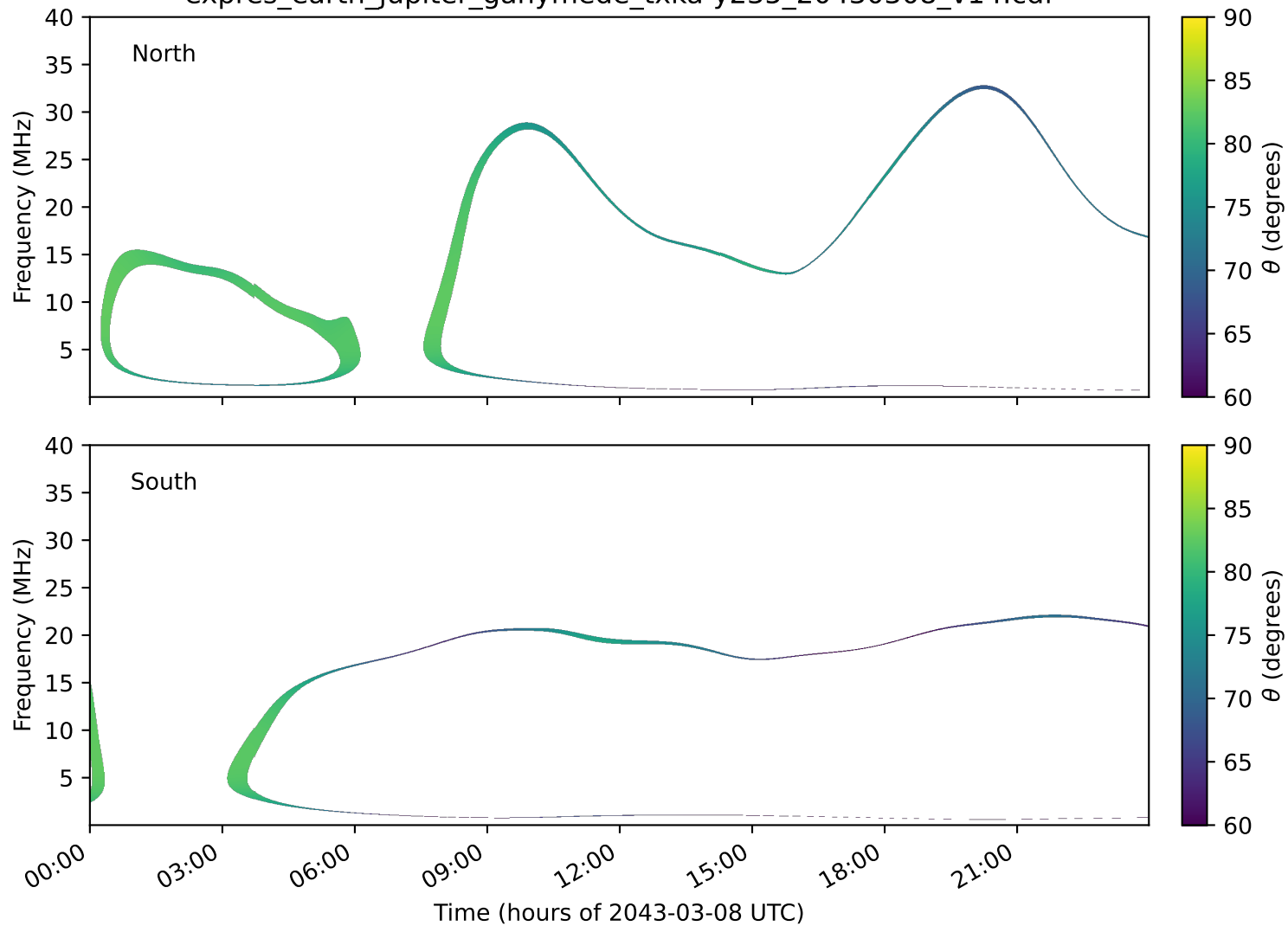
expres_earth_jupiter_ganymede_txka-y235_20430308_v14.cdf
