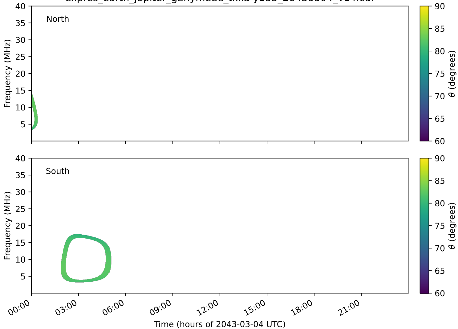
expres_earth_jupiter_ganymede_txka-y235_20430304_v14.cdf
