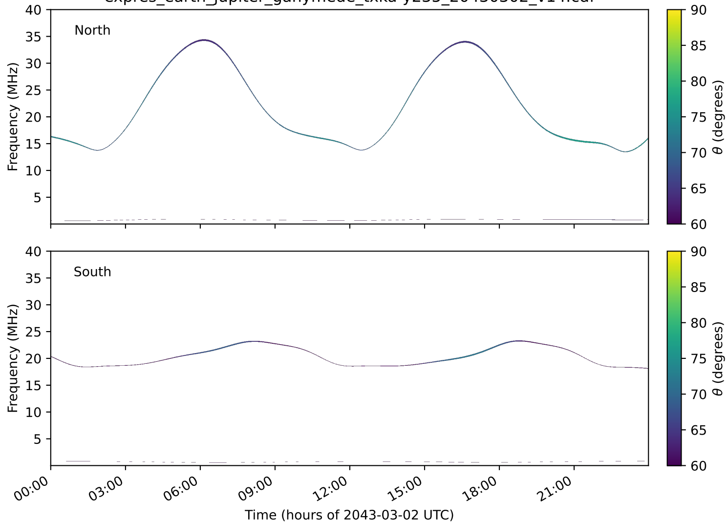
expres_earth_jupiter_ganymede_txka-y235_20430302_v14.cdf
