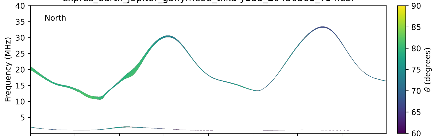
expres_earth_jupiter_ganymede_txka-y235_20430301_v14.cdf
