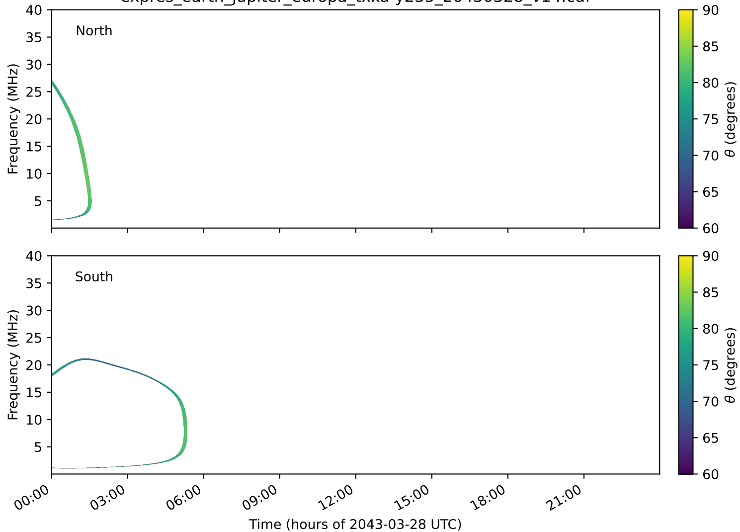
expres_earth_jupiter_europa_txka-y235_20430328_v14.cdf
