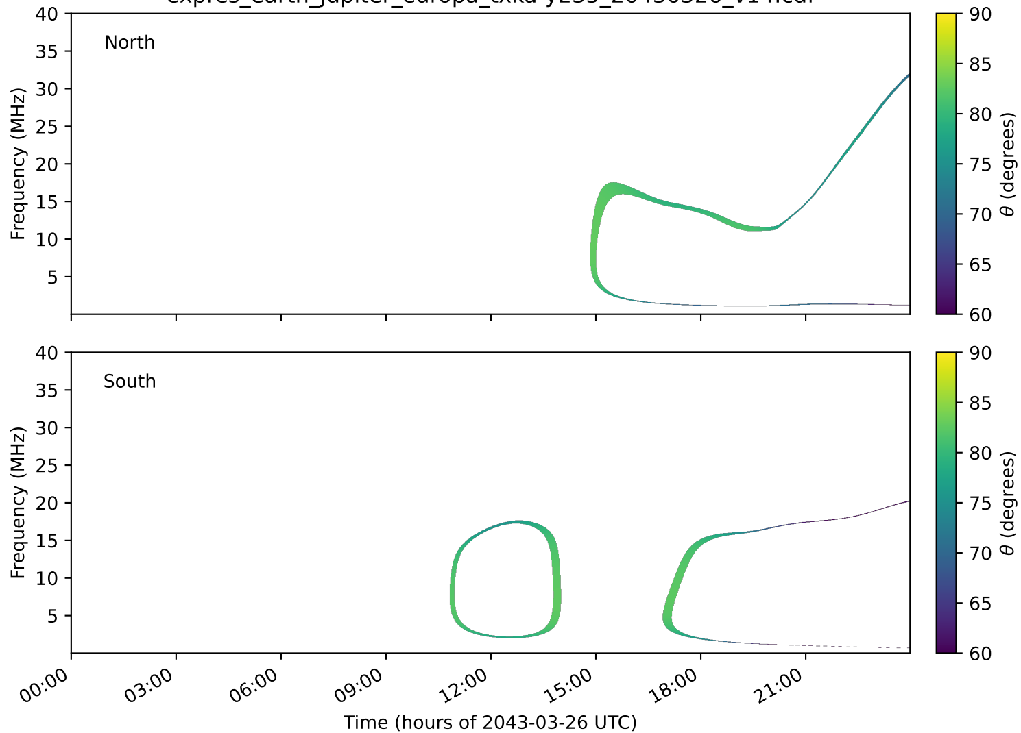
expres_earth_jupiter_europa_txka-y235_20430326_v14.cdf
