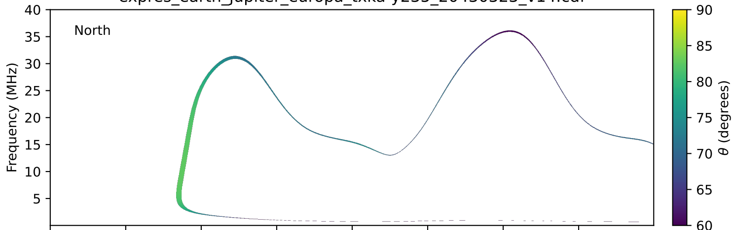
expres_earth_jupiter_europa_txka-y235_20430323_v14.cdf
