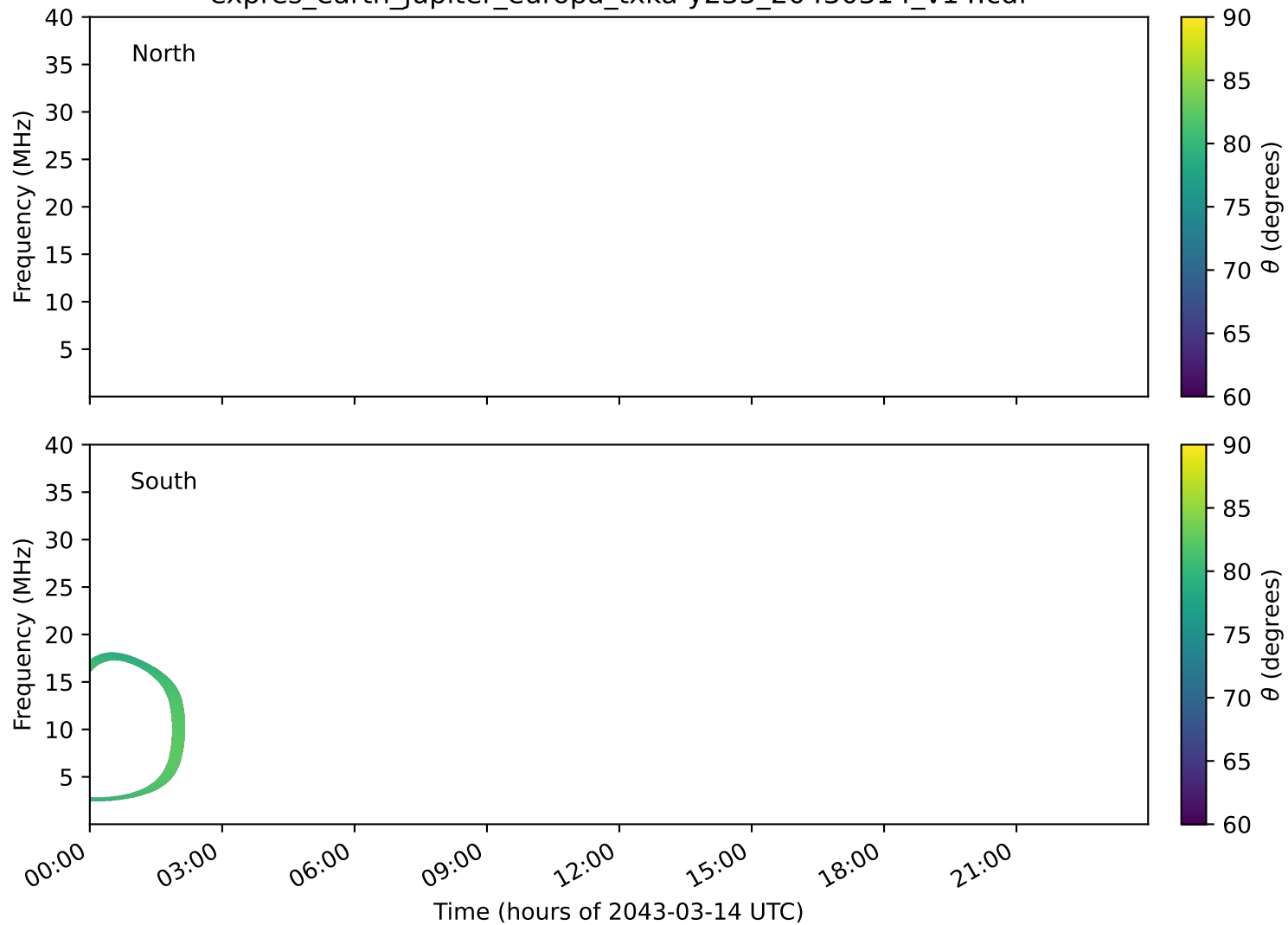
expres_earth_jupiter_europa_txka-y235_20430314_v14.cdf
