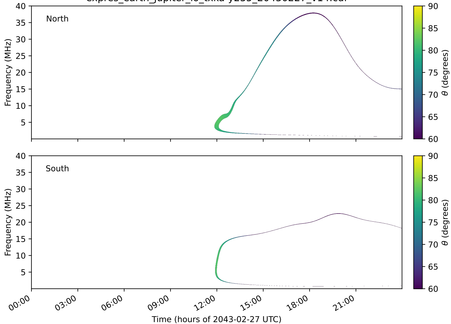
expres_earth_jupiter_io_txka-y235_20430227_v14.cdf
