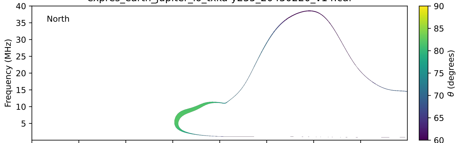
expres_earth_jupiter_io_txka-y235_20430220_v14.cdf
