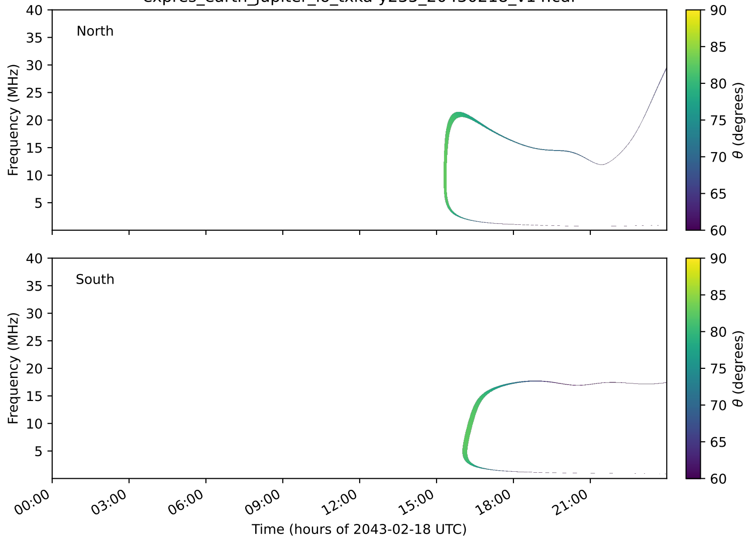
expres_earth_jupiter_io_txka-y235_20430218_v14.cdf
