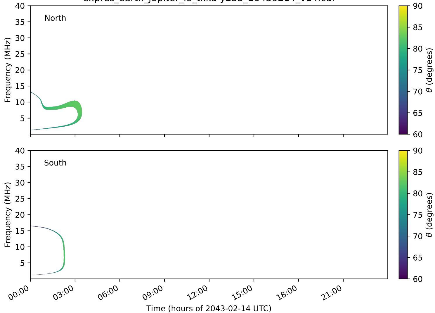
expres_earth_jupiter_io_txka-y235_20430214_v14.cdf
