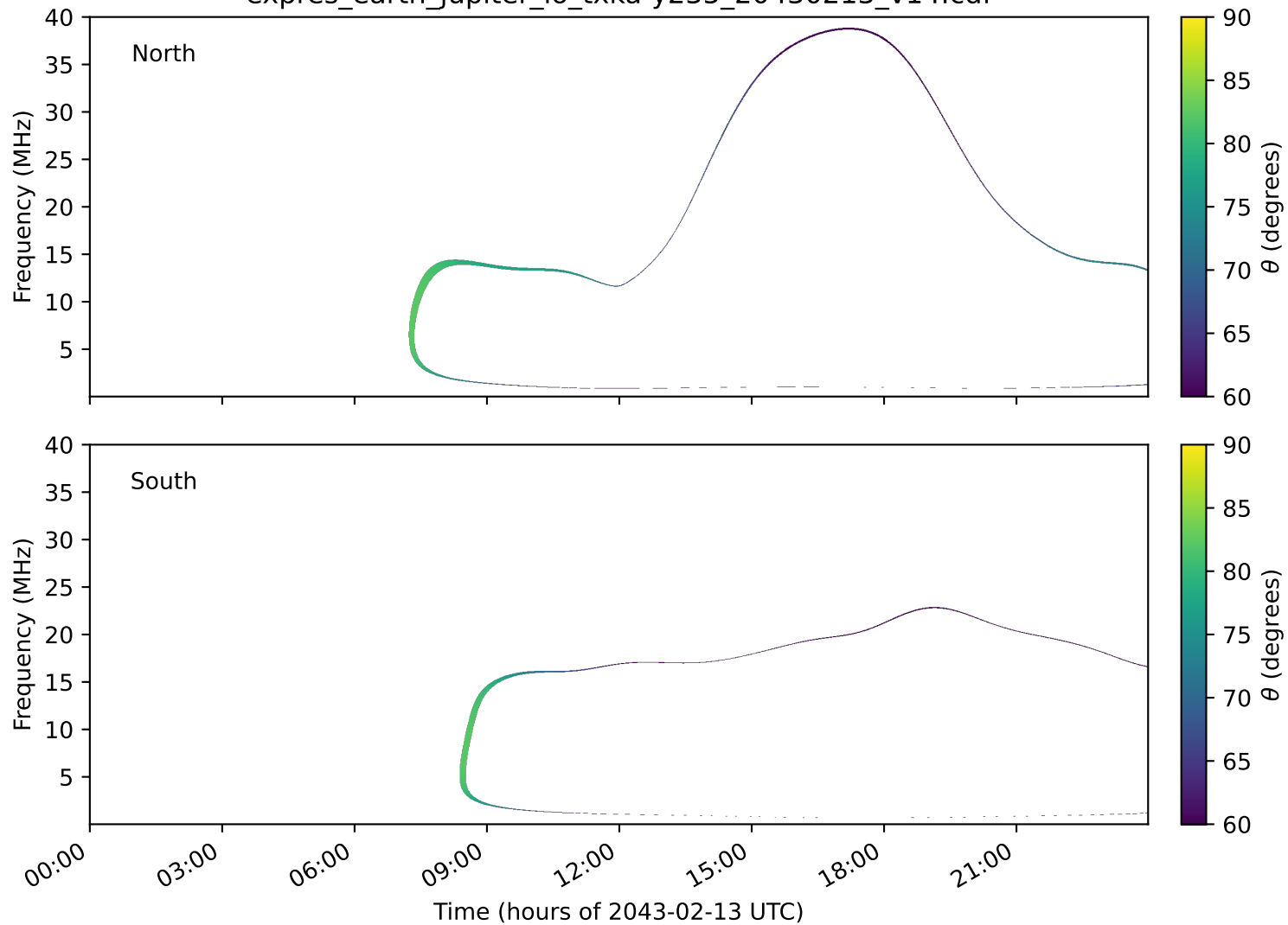
expres_earth_jupiter_io_txka-y235_20430213_v14.cdf
