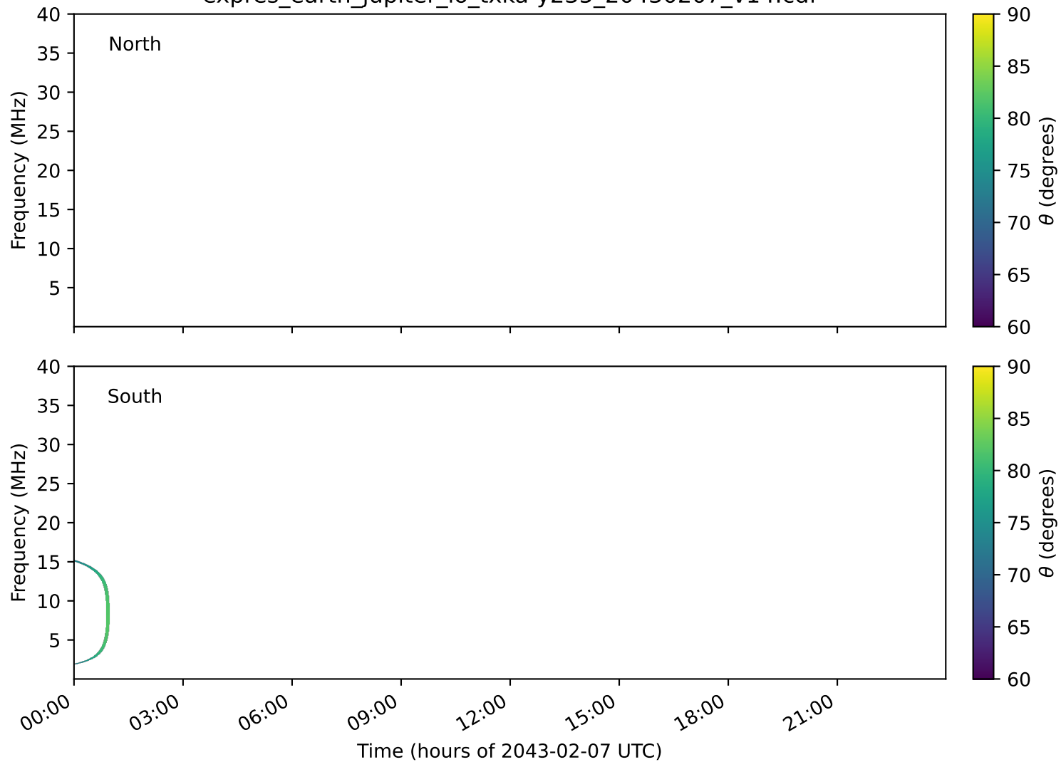
expres_earth_jupiter_io_txka-y235_20430207_v14.cdf
