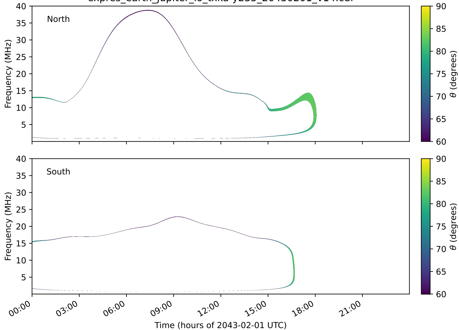
expres_earth_jupiter_io_txka-y235_20430201_v14.cdf
