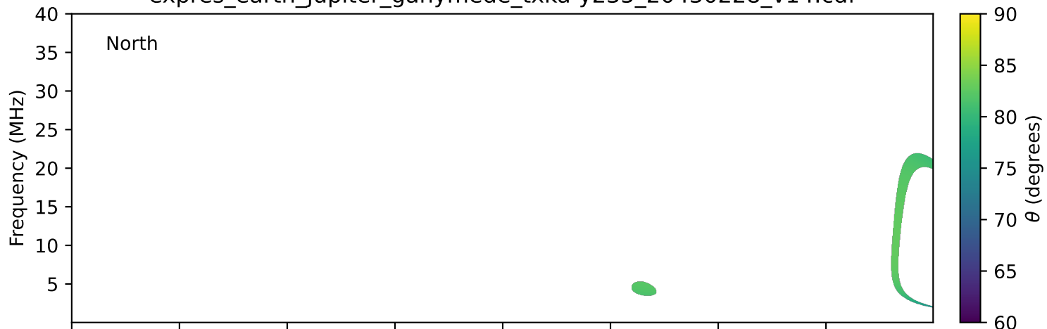
expres_earth_jupiter_ganymede_txka-y235_20430228_v14.cdf
