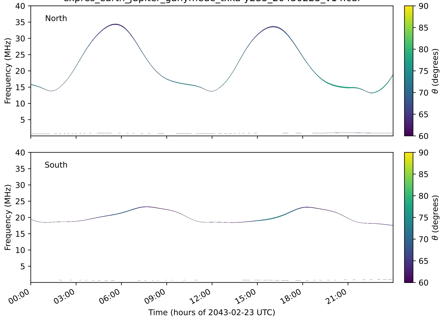
expres_earth_jupiter_ganymede_txka-y235_20430223_v14.cdf
