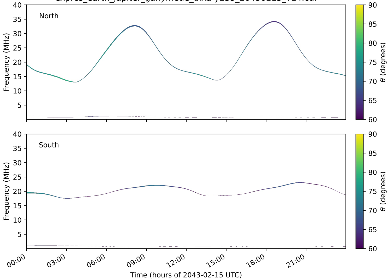
expres_earth_jupiter_ganymede_txka-y235_20430215_v14.cdf
