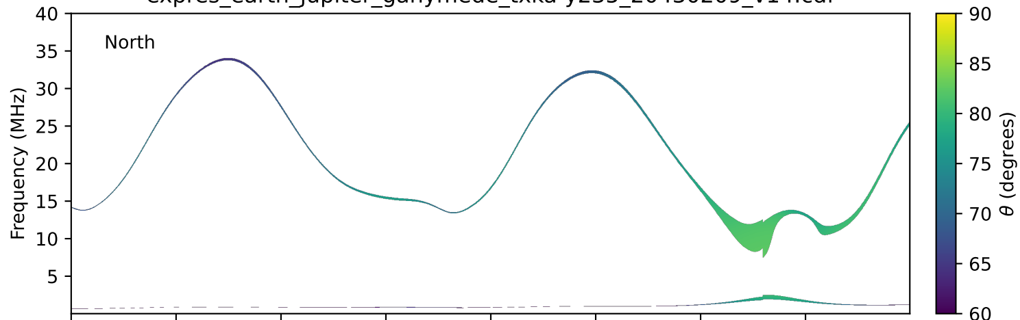
expres_earth_jupiter_ganymede_txka-y235_20430209_v14.cdf
