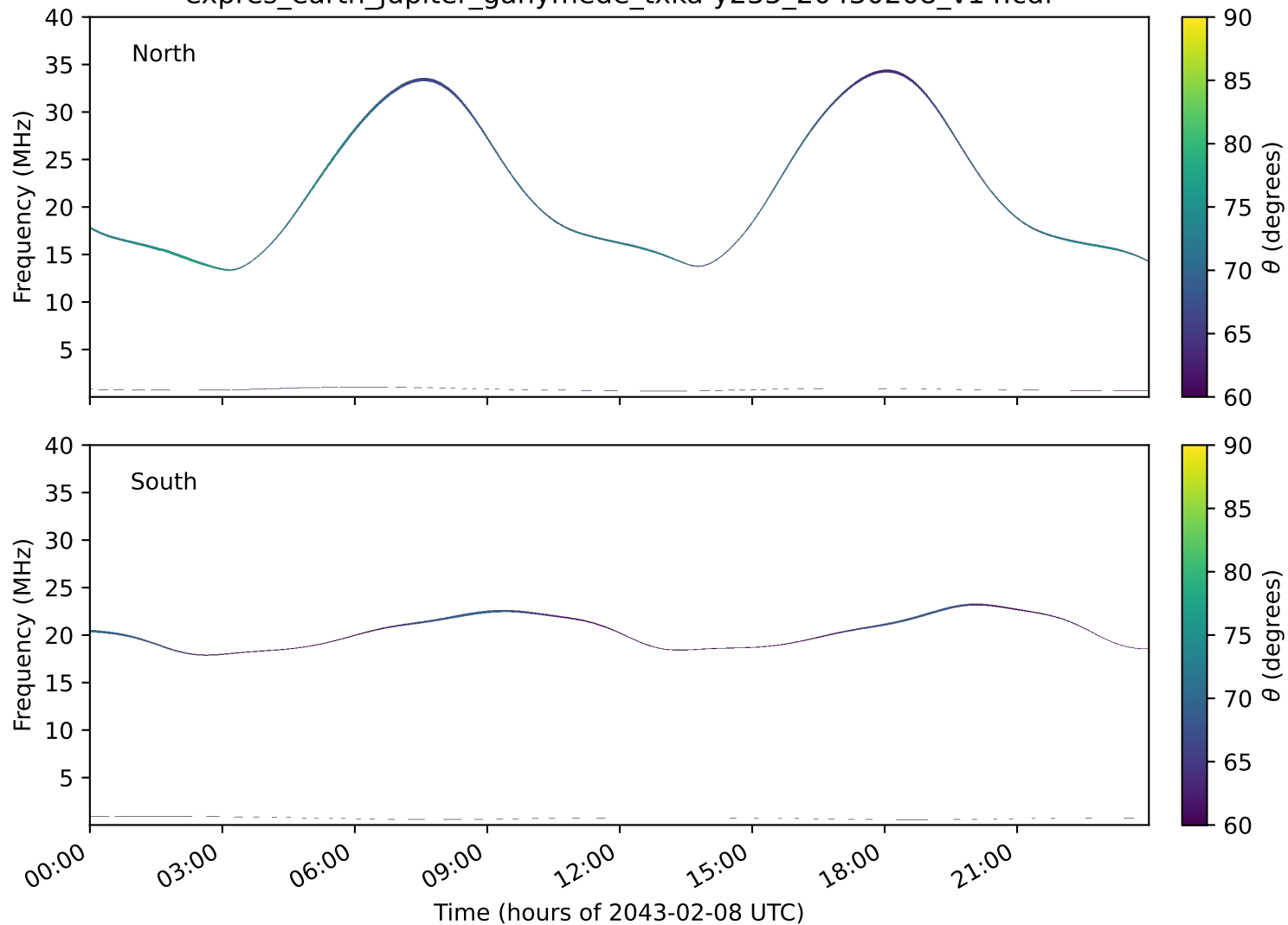
expres_earth_jupiter_ganymede_txka-y235_20430208_v14.cdf
