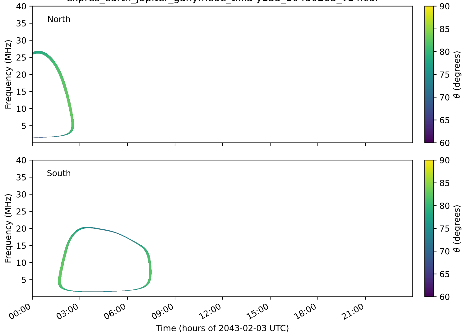
expres_earth_jupiter_ganymede_txka-y235_20430203_v14.cdf
