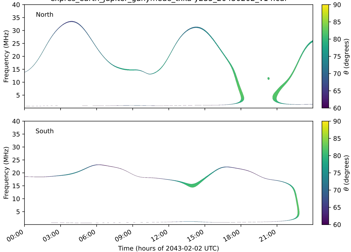
expres_earth_jupiter_ganymede_txka-y235_20430202_v14.cdf
