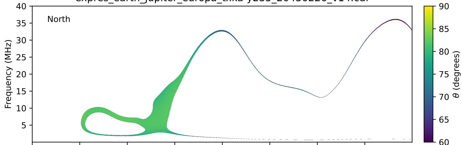
expres_earth_jupiter_europa_txka-y235_20430226_v14.cdf
