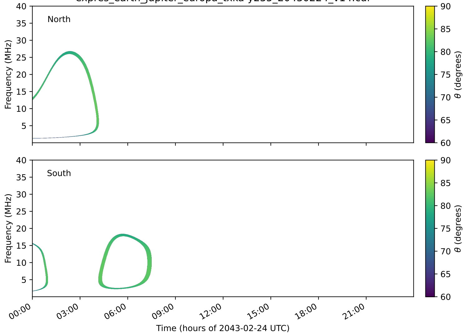
expres_earth_jupiter_europa_txka-y235_20430224_v14.cdf
