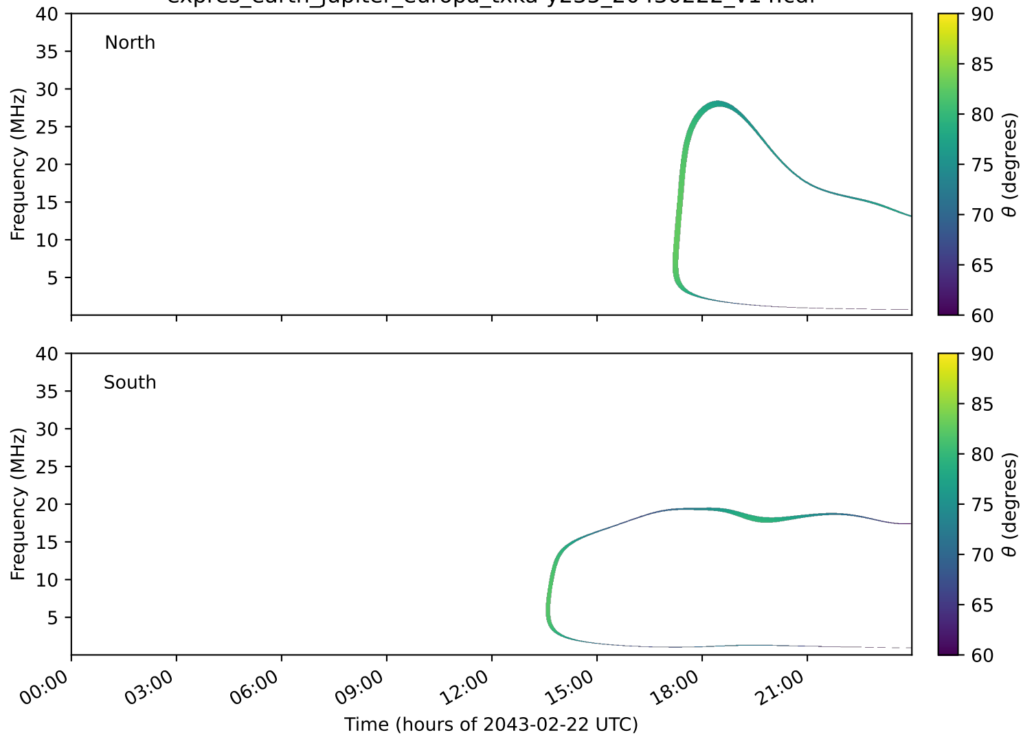
expres_earth_jupiter_europa_txka-y235_20430222_v14.cdf
