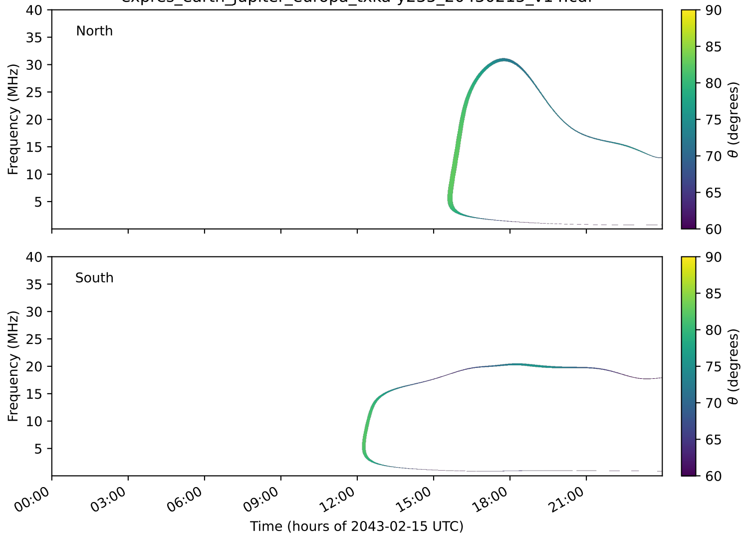
expres_earth_jupiter_europa_txka-y235_20430215_v14.cdf
