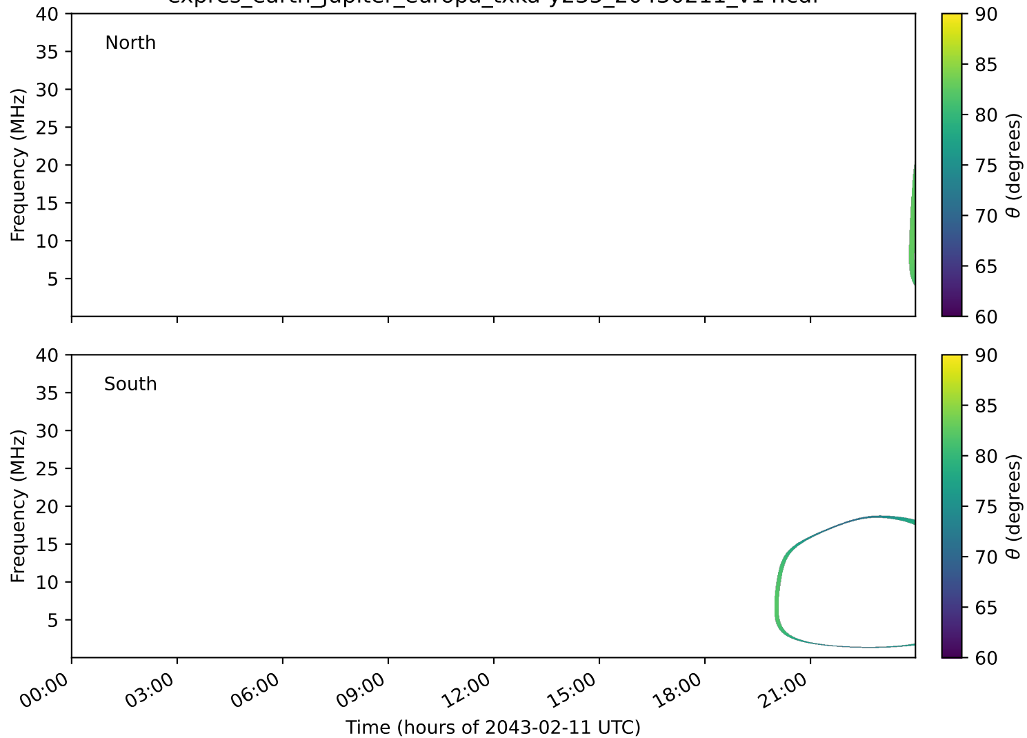
expres_earth_jupiter_europa_txka-y235_20430211_v14.cdf
