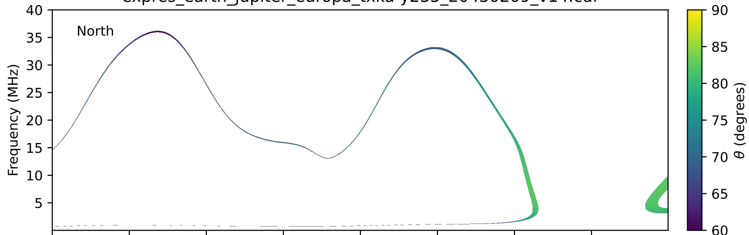
expres_earth_jupiter_europa_txka-y235_20430209_v14.cdf
