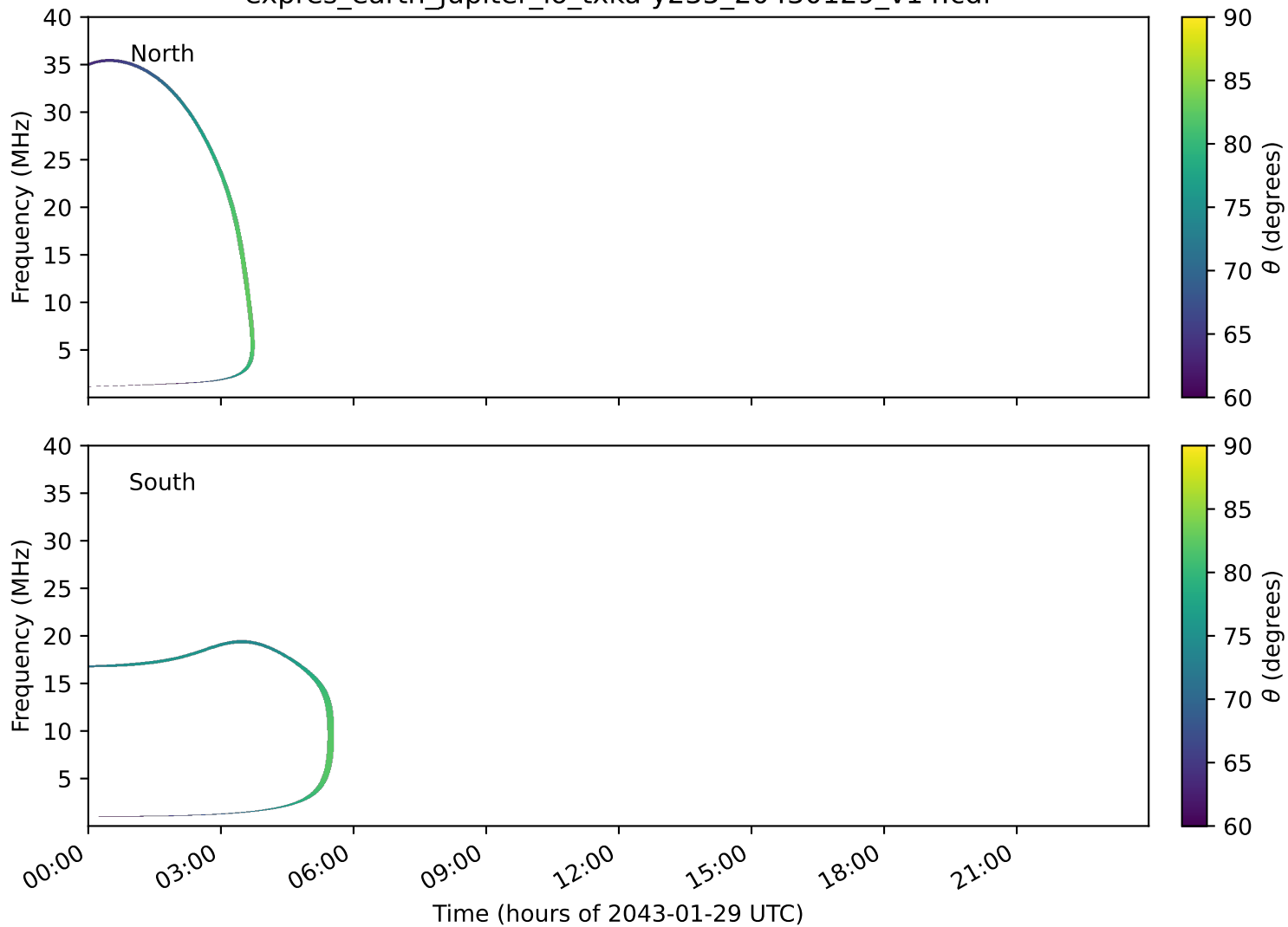
expres_earth_jupiter_io_txka-y235_20430129_v14.cdf
