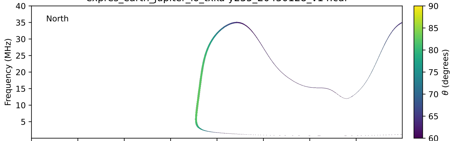
expres_earth_jupiter_io_txka-y235_20430128_v14.cdf
