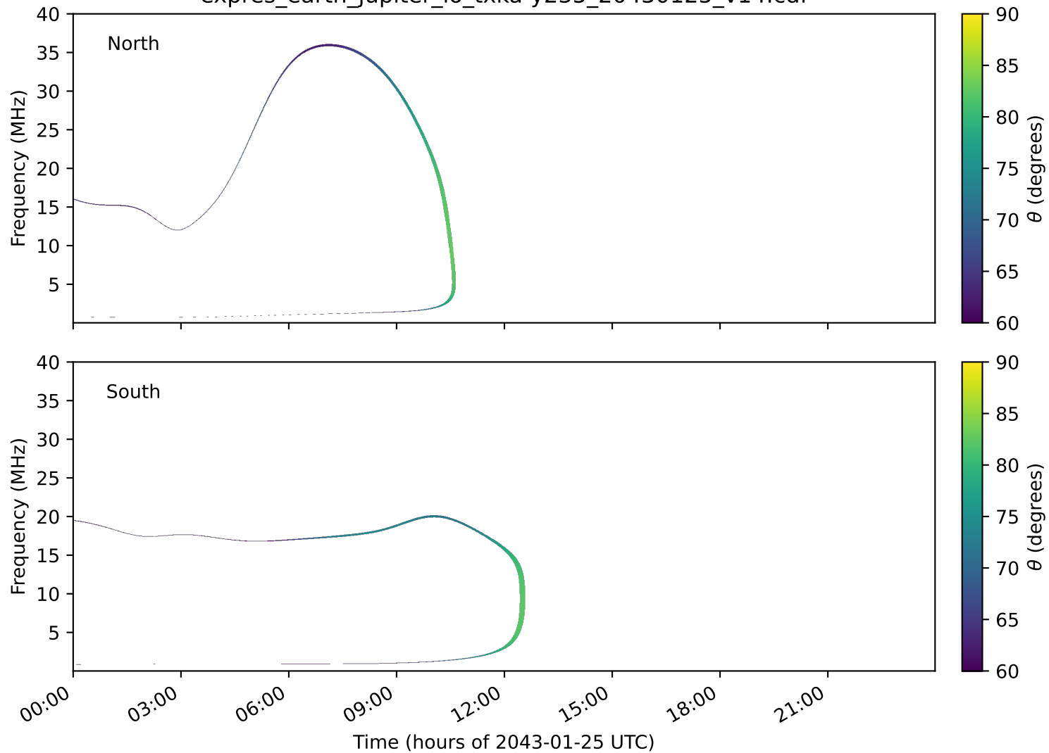
expres_earth_jupiter_io_txka-y235_20430125_v14.cdf
