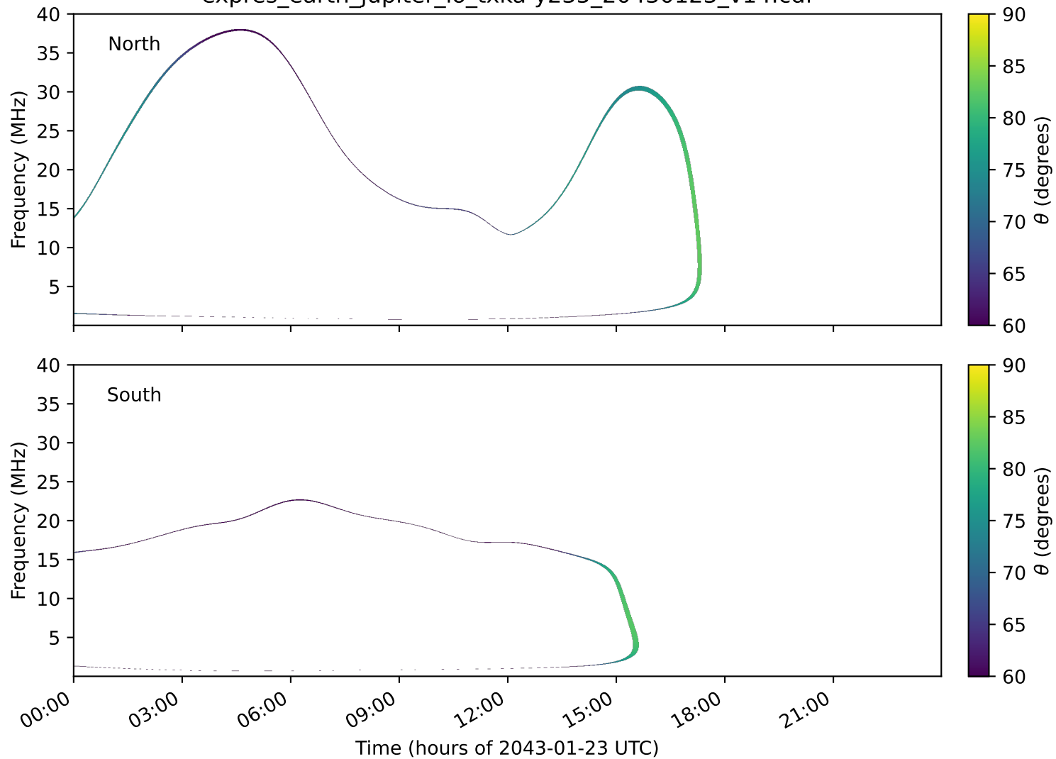
expres_earth_jupiter_io_txka-y235_20430123_v14.cdf
